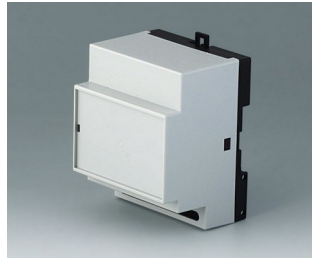
B6513111 RAILTEC B, 4 modules, Vers. XI PC (UL 94 V-0) light grey RAL 7035 70x86x58mm
